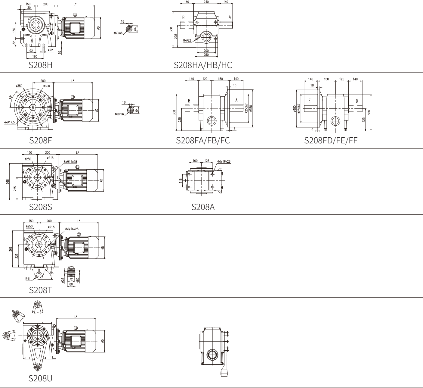
MP motor dimension for S208
