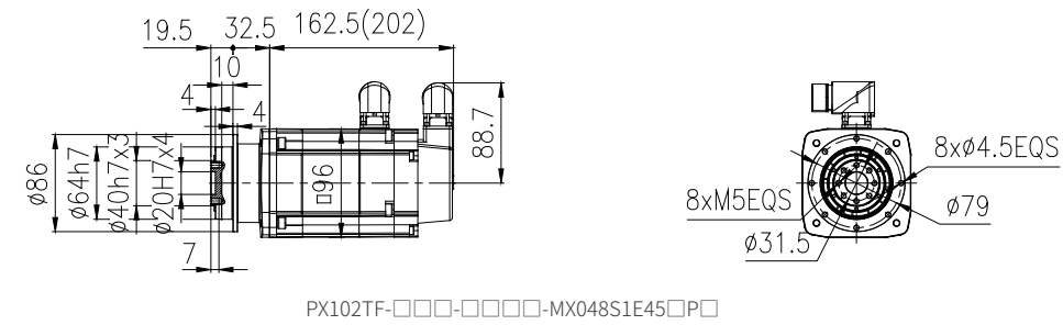
MX048S Outline dimension diagram (mm)
