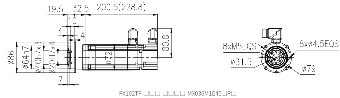
MX036M Outline dimension diagram(mm)
