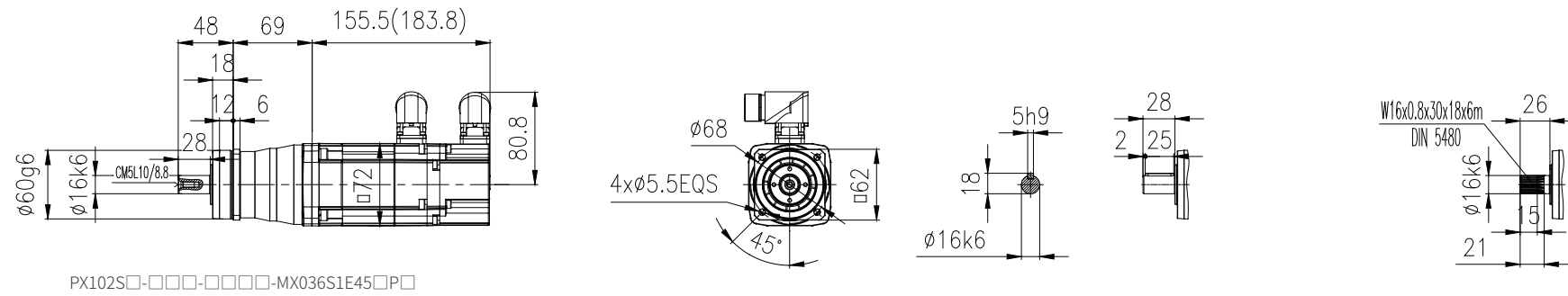
MX036S Outline dimension diagram(mm)
