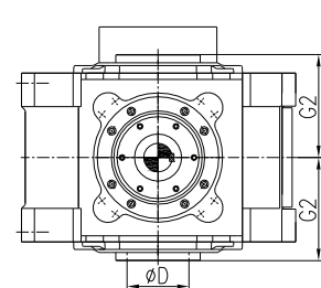
B3..VH Parallel key hollow shaft
