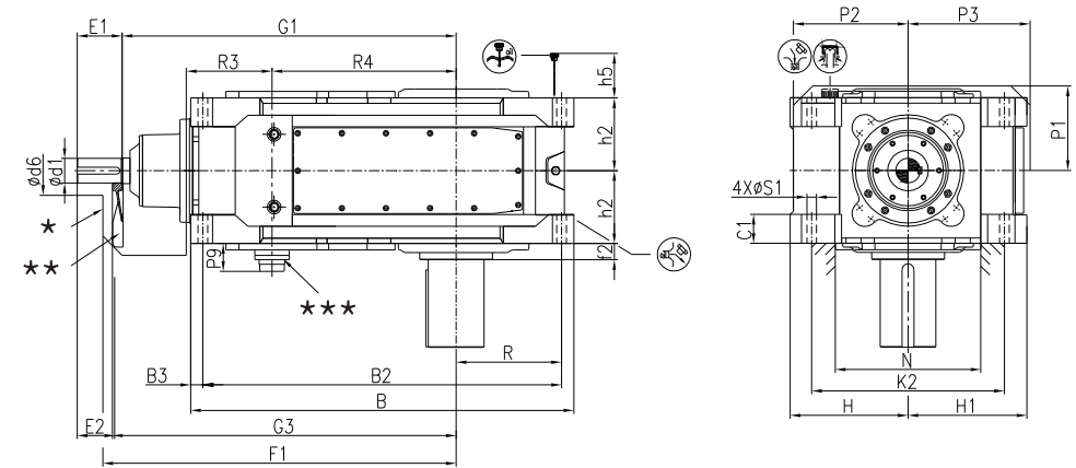
B3..VH Parallel key hollow shaft
