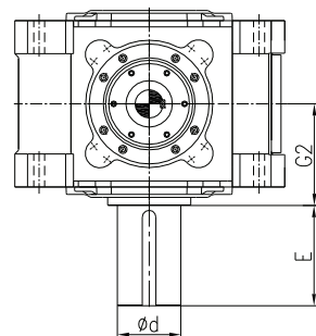
B3..VS Parallel key solid shaft
