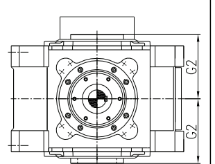
B3..VK Hollow shaft with involute spline
