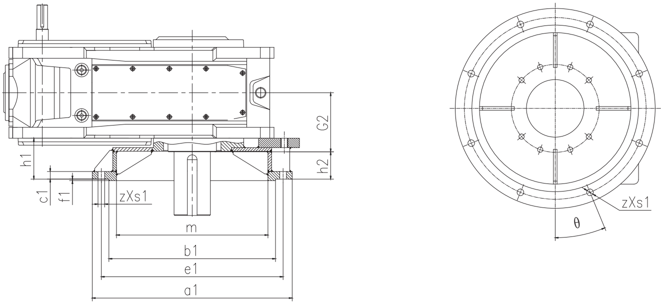
16.9 输出安装法兰 (附件代号:UF32) 16.9 Outpt mounting flange (Code:UF32)
