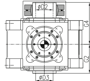
B3..VD Hollow shaft with shrink disc
